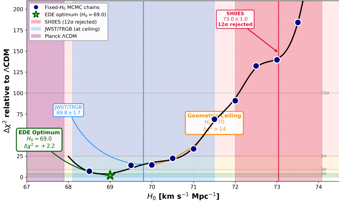
Figure 7: Profile likelihood for H_0 in the Geometric EDE model. Each point represents a fixed- H_0 MCMC chain with all other parameters free. The profile is nearly flat near H_0 \approx 69 \text{ km s}^{-1} \text{ Mpc}^{-1} (green star), then rises sharply beyond \approx 70 . Shaded bands show external constraints: Planck \Lambda CDM (purple), JWST/TRGB (blue), and SH0ES (red). The SH0ES value lies far above the geometric ceiling imposed by CMB+BAO.
